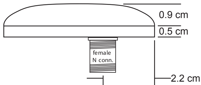
Indoor retransmit antenna (passive)
