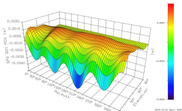
Figure 14 – Phase center variation at L1. Same results have been observed at G1.
