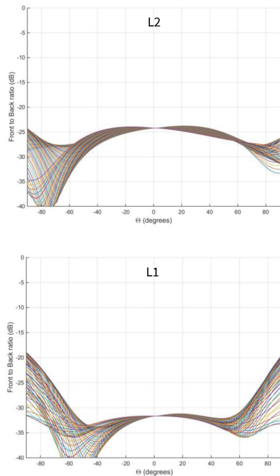
Figure 9 – Down-Up Ratio of the VP6000 at L2 and L1 on 60 azimuth cuts.
