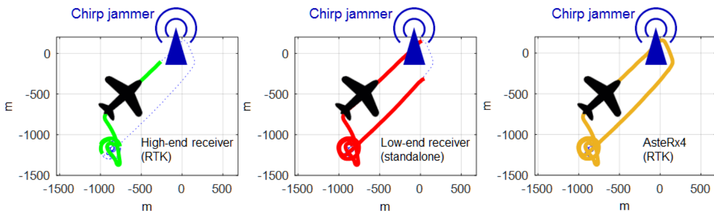
Figure 2: RTK position availability for the AsteRx4 with AIM+ activated and a comparable high-end receiver. The low-end receiver tracks L1 only and outputs less-precise standalone positions. A 10mW chirp jammer is located on the ground at position (0,0) as shown.
