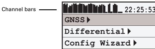
Figure 3-2: R330 menu
