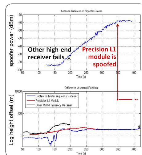
FIGURE 4: Height plot comparison for three different receivers subject to spoofing as the spoofer power is increased. The Septentrio AsteRx4 position survives to maximum spoofer power thanks to frequency diversity.
